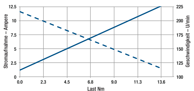
K2RAG20-24VDC
