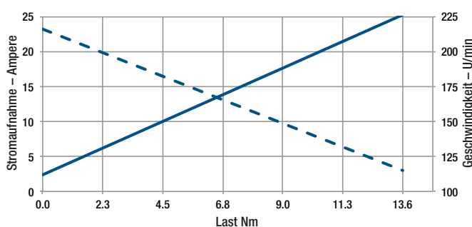
K2RAG20-12VDC
