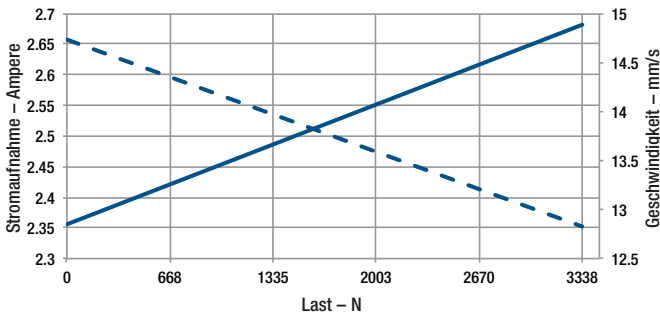
K2G20-115VAc
