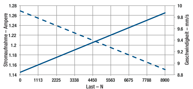
K2xG30-230VAc
