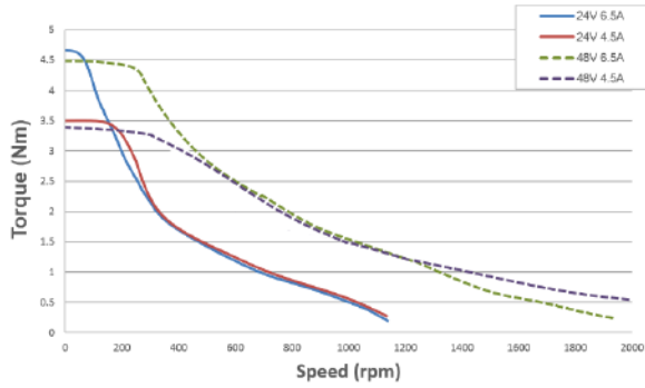
NEMA 34 Medium (IP20)
