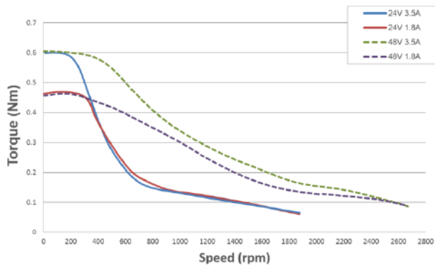
NEMA 17 Medium (IP20)
