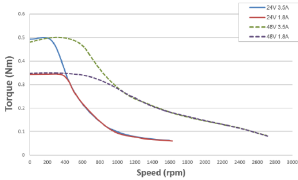
NEMA 17 Short (IP20)
