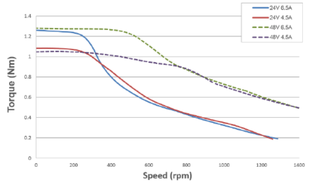
NEMA 23 Short (IP20, IP65)
